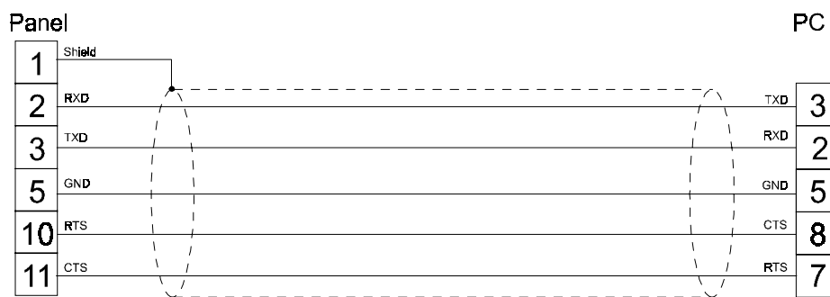
figure 1. Cable diagram
