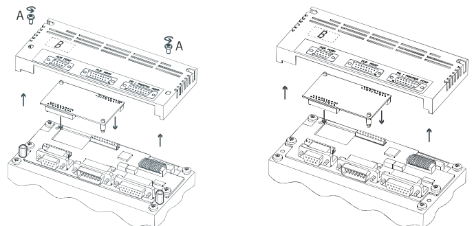
Figure 2 – Mounting TCM09 board/ TCM09 Montage/ TCM09 montage/ TCM09 montaje/ Montaggio modulo TCM09.
