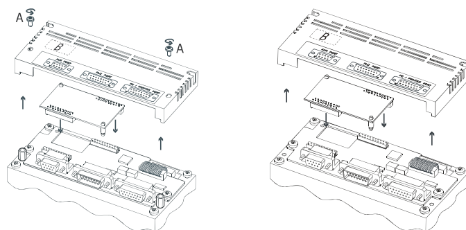
Figure 2 – Mounting TCM15 board/ TCM15 Montage/ TCM15 montage/ TCM15 montaje/ Montaggio modulo TCM15.
