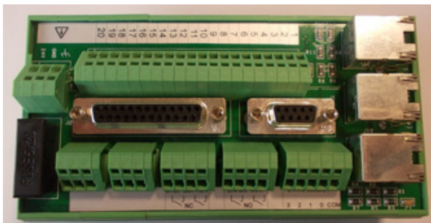
Figure 12: Cable splitter
