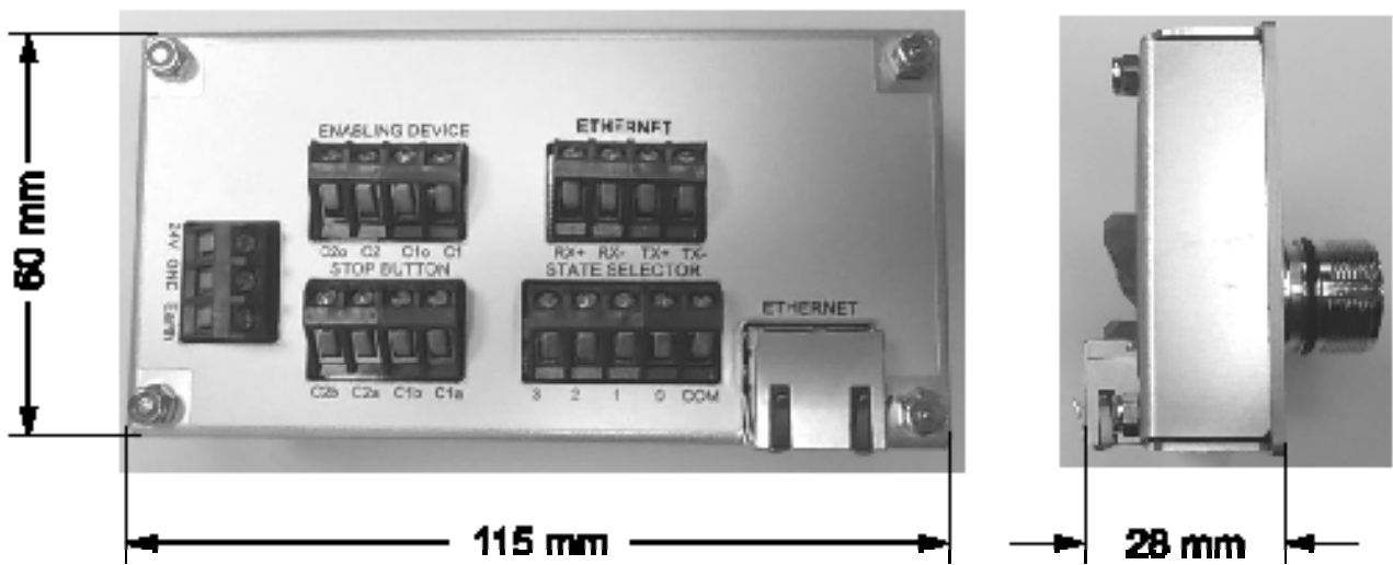
Figure 16: Connection Box dimensions
