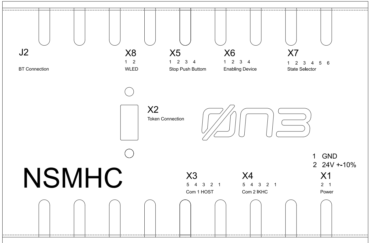
Figure 2.16: NSMHC connectors
