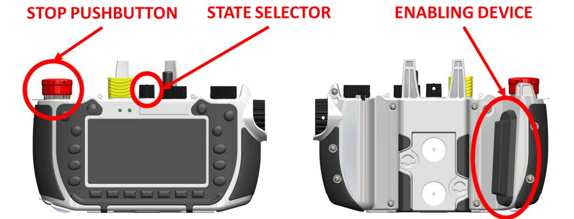
Figure 2.6: Safety related devices position
