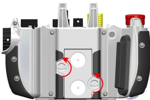
Figure 2.9: Battery replacement
