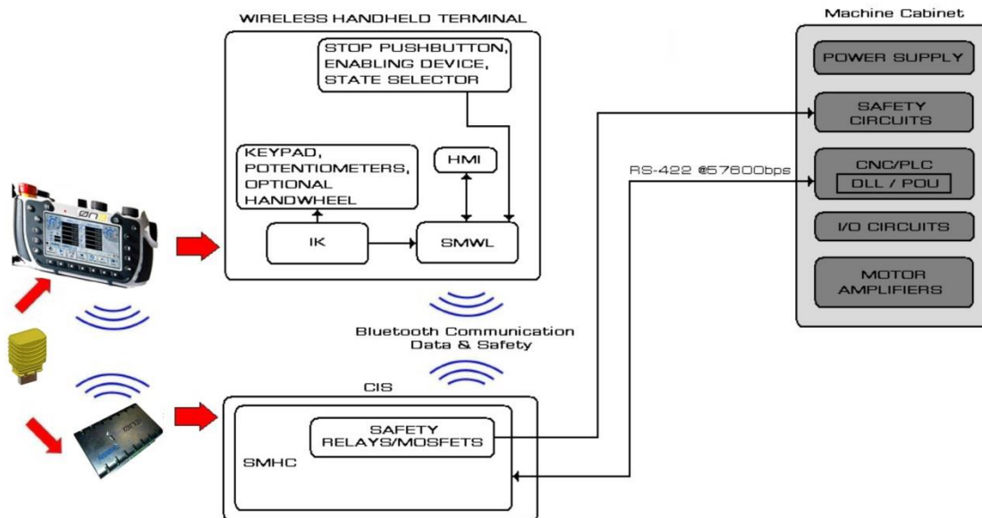
Figure 3.1: Architecture Overview
