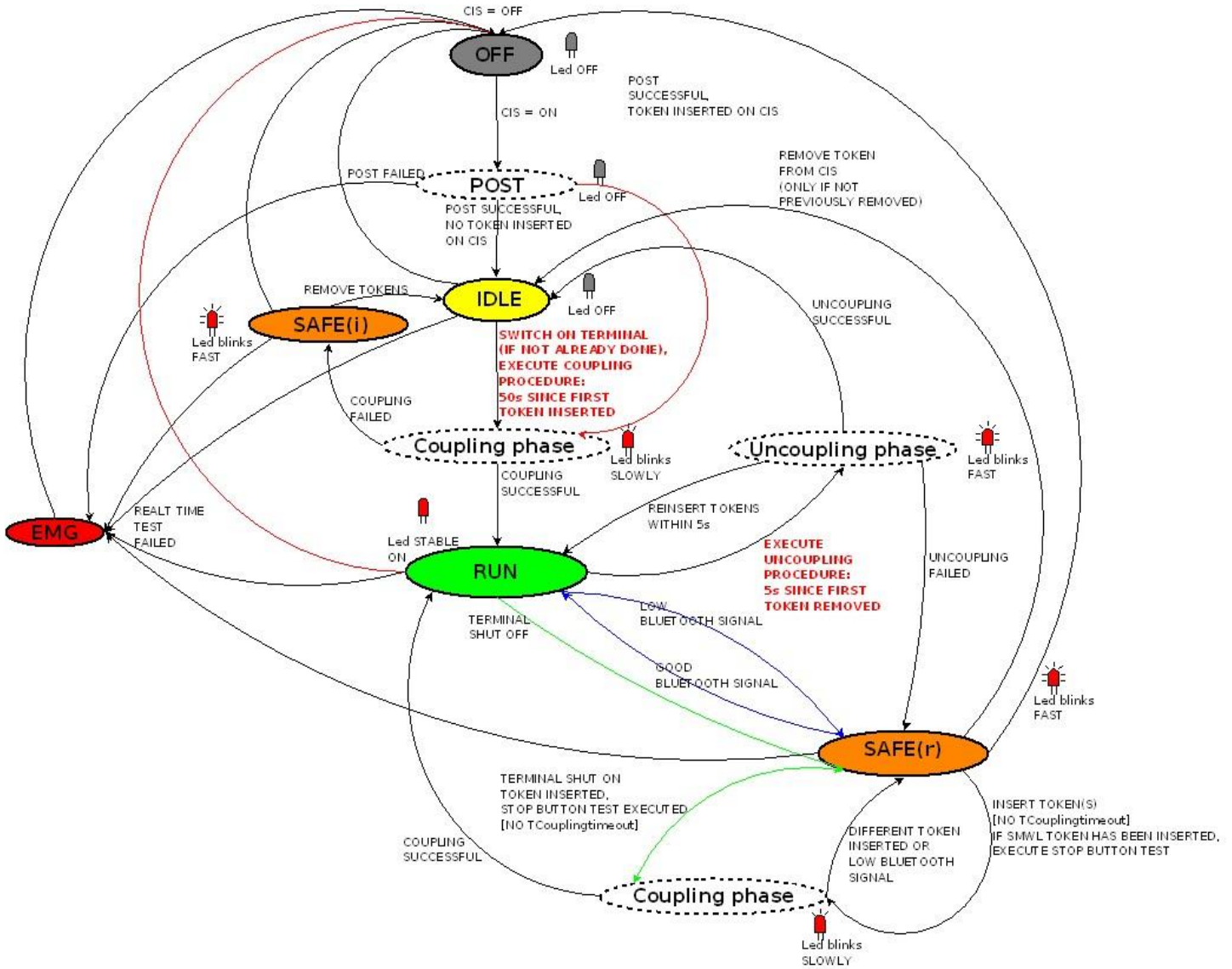
Figure 3.2: Safety system status diagram
