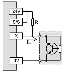
NPN (sink)
