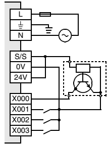
Transmisor NPN (sink)
