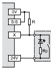
Circuito a logica positiva PNP (Source)
