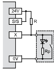
NPN (sink)
