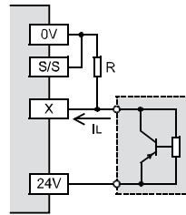
PNP (source)
