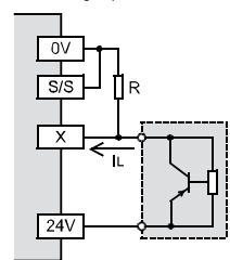
Circuito a logica positiva PNP (Source)
