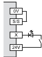
PNP (source)
