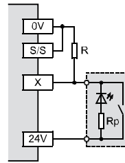
PNP (source)
