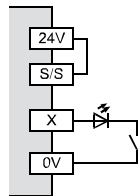
NPN (sink)
