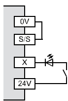
Circuito a logica positiva PNP (Source)
