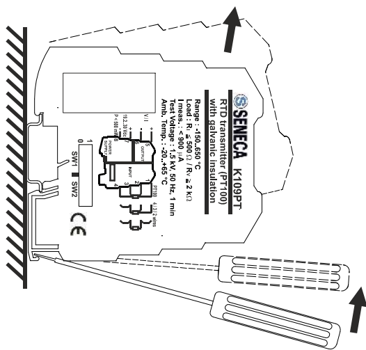
Removing the module from the rail
